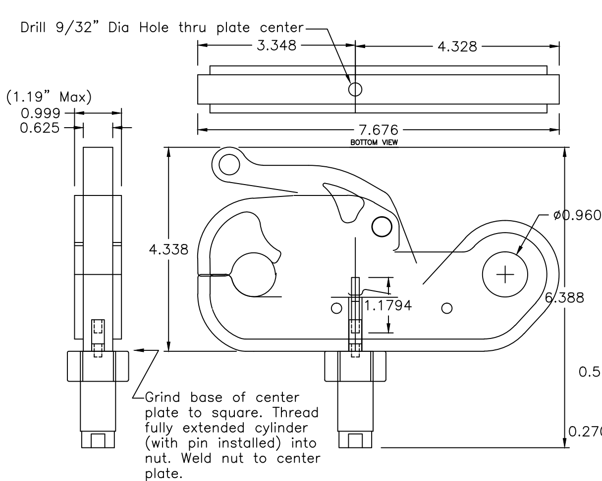
Assembly End View
