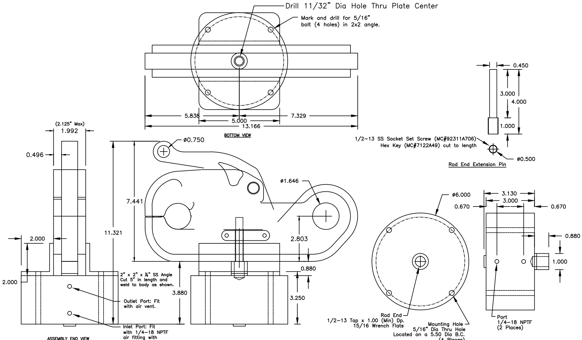
SEA CATCH TR11AIR ASSEMBLY
